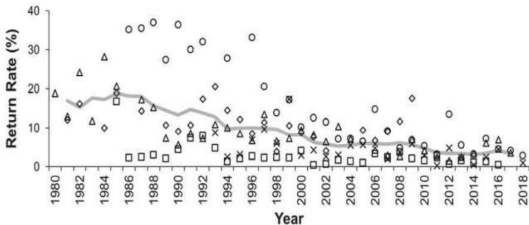
Figure 14. Return rates (%) of wild adult Atlantic salmon to southern European Rivers from 1980 to 2018, North Esk River, Scotland (◇), River Bush, Northern Ireland (○), Corrib River, Ireland (Δ), River Dee, Wales (x) and Rivière Nivelle, France (□); and three-year rolling average of all return rates (gray line). Data adapted from ICES (2015, 2020).
